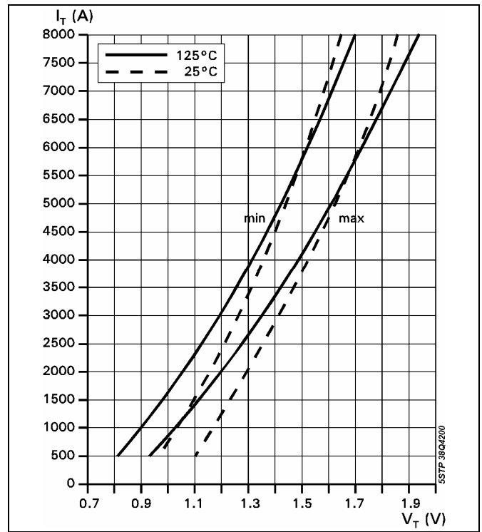
Fig. 3 On-state characteristics, T_j = 125^\circ\text{C} , 10ms half sine
