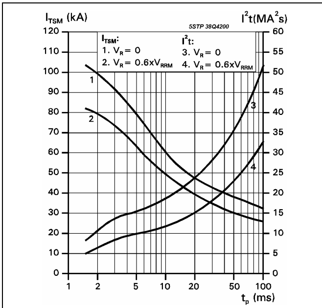
Fig. 6 Surge on-state current vs. pulse length, half-sine wave
