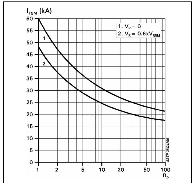
Fig. 7 Surge on-state current vs. number of pulses, half-sine wave, 10 ms, 50Hz
