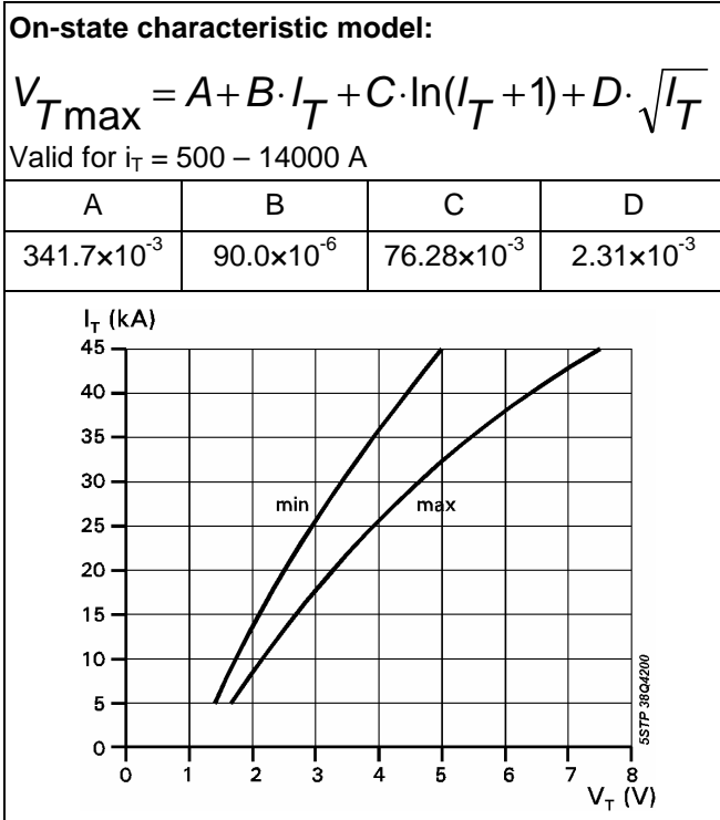
Fig. 2 On-state characteristics
